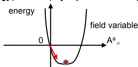
Energy(Potential) by Equivalent Principle
