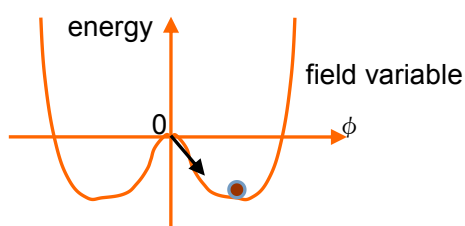
Higgs Model Energy(Potential)
